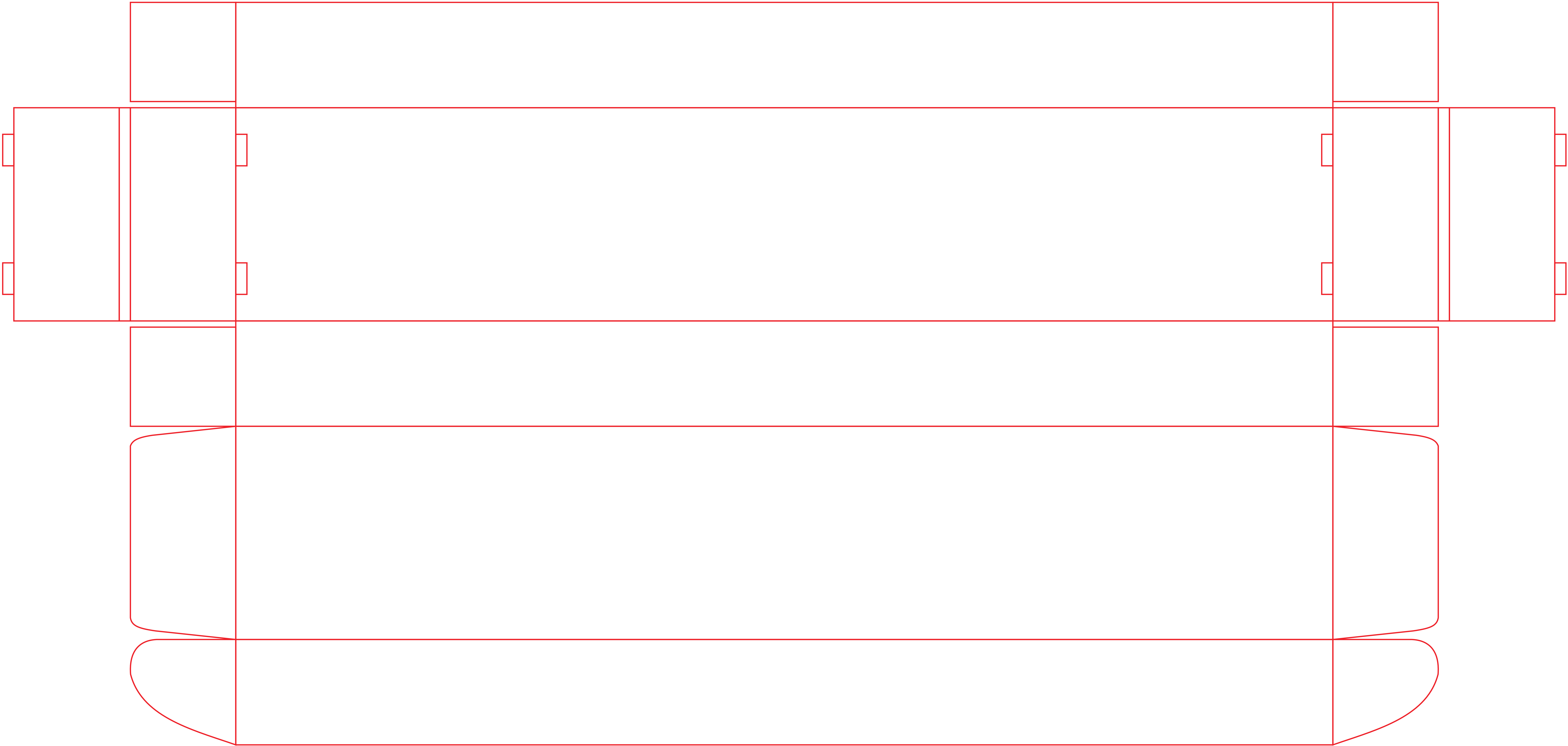
PLB147XL:885x172x85mm
